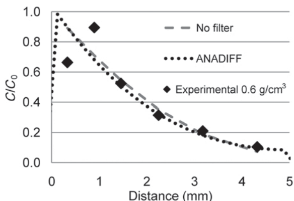
Figure 5. Experimental gold concentration profile in bentonite at dry density 0.6 \text{ g/cm}^3 from the 2-nm diffusion experiment and corresponding modeled profiles. Black diamonds show the experimental points. The dashed gray curve shows the modeled curve without filter effects. The dashed black curve shows the concentration profile using ANADIFF .
