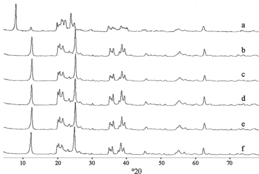
Figure 1. WXR of kaolinite precursors with single intercalation agents: (a) Kao-DMSO; (b) Kao-KAc; (c) Kao-NaAc; (d) Kao- NH_4Ac ; (e) Kao-Urea; and (f) Kao-DMF.
