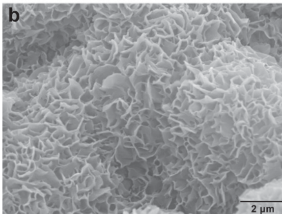
Figure 5. (a) Etched cpx ( \sim\text{Wo}_{38}\text{En}_{41}\text{Fs}_{21} = diopside augite) (top left background) with 'cornflake' smectite (neofformed?) bottom right foreground. (b) Closeup of 'cornflake' smectite. MSU CAM JEOL 6400 SEM.
