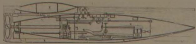
DAVIES. — 1883.
