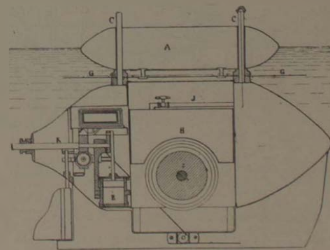
SMITH. — 1873.
