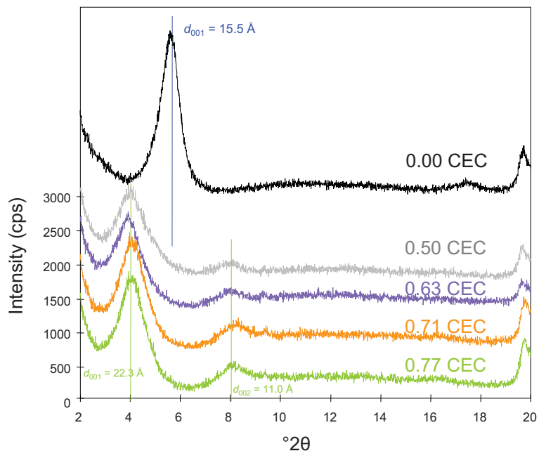
Figure 8. XRD patterns of SAz-1 intercalated with different amounts of TC at pH 4–6.
