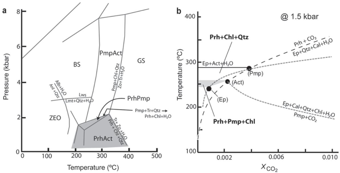
Figure 9. (a) Phase diagrams indicating prehnite stability as functions of temperature and pressure. Metamorphic facies (ZEO = zeolite, GS = greenschist, BS = blueschist) are indicated and selected reactions are shown (adapted from Schiffman and Day, 1999). (b) Temperature and mole fraction of CO 2 (adapted from Robinson and Bevens, 1999). Prh = prehnite, Pmp = pumpellyite, Chl = chlorite, Anl = analcime, Qtz = quartz, Alb = albite, Lws = lawsonite, Zo = zoisite, Tr = tremolite, Ep = epidote, Act = actinolite, Cal = calcite.
