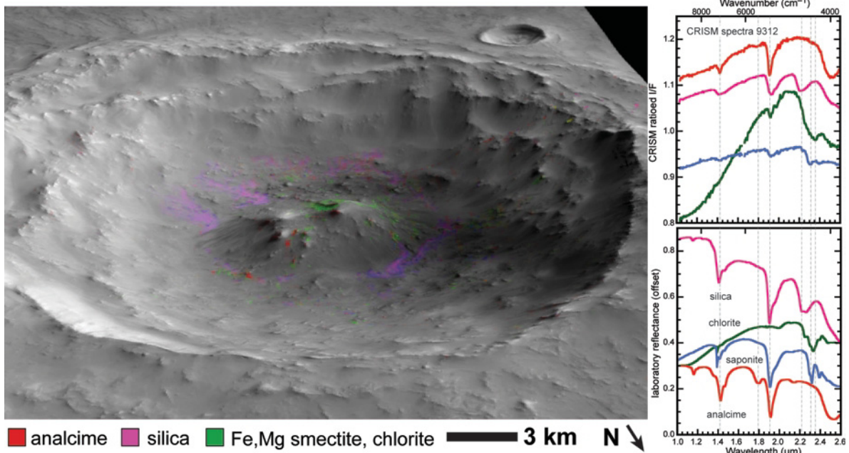
Figure 5. Analcime, silica, Fe,Mg-smectite, and chlorite have been identified in a 25 km impact crater in northern Syrtis Major (20°N, 66°E). CRISM mineral maps were constructed from the band depth at 2.5 \mu\text{m} (red), 2.3 \mu\text{m} (green), and 2.2 \mu\text{m} (blue) and the color mapping of minerals verified by comparing CRISM spectra to data from spectral libraries (Clark et al. , 2007). The maps were then overlain on a CTX image mosaic and draped over a MOLA-derived digital elevation model. In this color combination and display stretch, Fe,Mg-smectites and chlorite are both mapped in green, analcime is red, and silica is blue to magenta.
