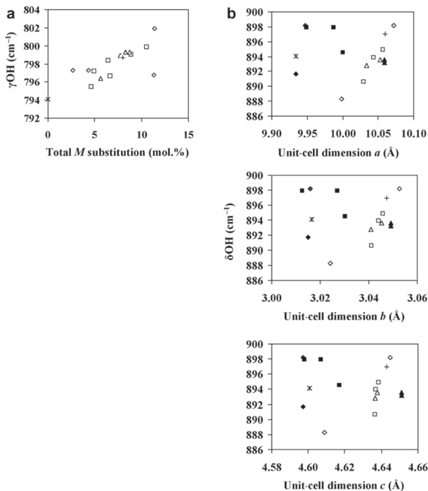
Figure 3. (a) Linear ( r^2 = 0.82 ) relationship of out-of plane ( \gamma_{OH} ) bending frequency with total substitution in goethite (* pure, \diamond single metal, \square two metals, \triangle three metals, and + four metals substituted goethite.). The r^2 values are provided excluding the single Zn-substituted sample. (b) Linear ( r^2 = 0.69-0.92 ) relationship of in-plane ( \delta_{OH} ) frequency of single Cd- and Zn- and multi-metal (Cr,Zn, Zn,Cd, Zn,Pb, Cr,Zn,Pb, Zn,Cd,Pb, and Cr,Zn,Cd,Pb)-substituted goethite having unit-cell dimensions: a > 10.00 \text{ \AA} , b > 3.03 \text{ \AA} , and c > 4.62 \text{ \AA} . Pure goethite and Cr-, Pb-, Cr,Cd-, Cr,Pb-, and Cd,Pb-substituted goethites having unit-cell dimensions less than the above-mentioned limits and Cr,Zn,Pb and Cr,Cd,Pb having dimensions greater than the above-mentioned do not follow the linear trend (shown with solid symbols for metal-substituted goethite).
