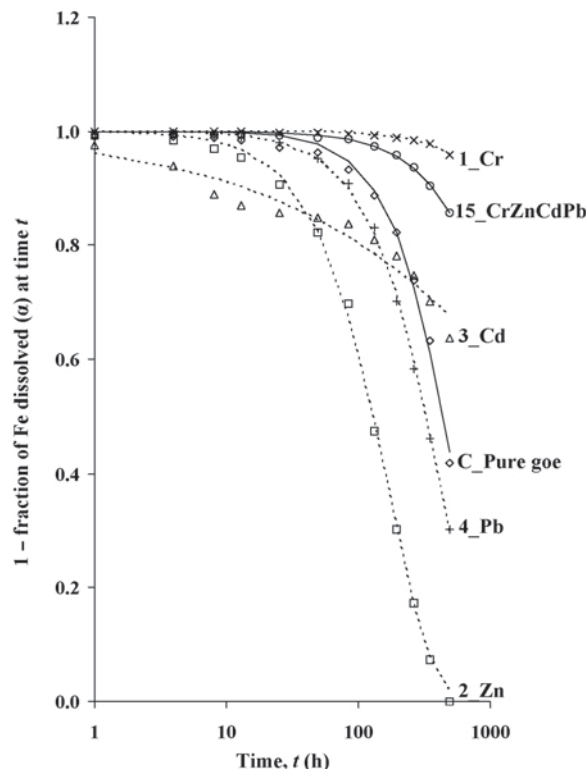
Figure 7. Kabai plots for synthetic single- and tetra-metal (Cr, Zn, Cd, and Pb)-substituted and pure goethites.
