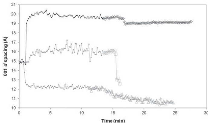
Figure 5. Movement of the 001 reflection of NAu-2 on reaction with: (1) H 2 O (black diamonds), (2) low acid solution (light gray squares), and (3) high acid solution (mid-gray triangles) at room temperature (solution injection: small, solid symbols) and 125°C (slurry: large, open symbols). (Note only every fifth data point has been plotted for clarity.)
