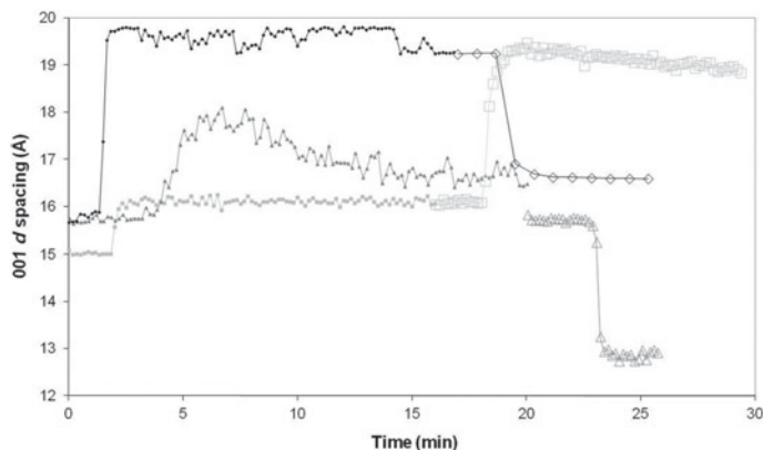
Figure 4. Movement of the 001 reflection of NAu-1 on reaction with: (1) H 2 O (black diamonds), (2) low acid solution (light gray squares), and (3) high acid solution (mid-gray triangles) at room temperature (solution injection: small, solid symbols) and 125°C (slurry: large, open symbols). (Note only every fifth data point has been plotted for clarity.)
