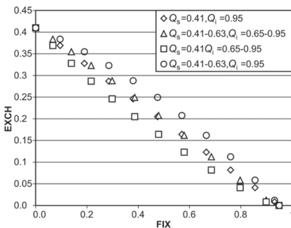
Figure 4. Relations between fixed (FIX) and exchangeable (EXCH) cations per \text{O}_{10}(\text{OH})_2 , modeled using equations 2 and 3 for stable and variable Q_i and Q_s .
