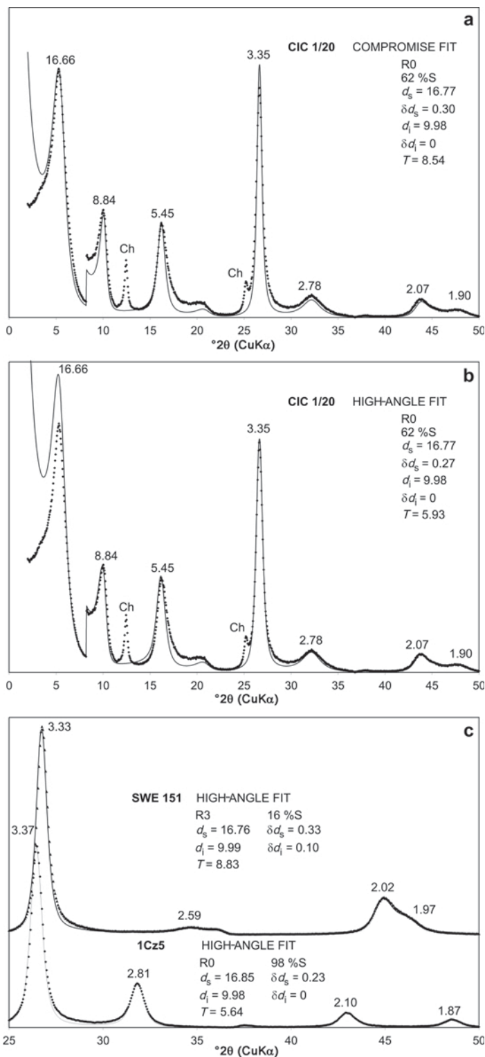
Figure 8. Examples of SYBILLA models and experimental XRD patterns of glycolated, \text{Ca}^{2+} -saturated I-S. Comparison of two models for sample CIC 1/20 (chlorite peaks not modeled): (a) 'compromise fit' based on the entire angular range; (b) 'high-angle fit' employing peaks >26^\circ 2\theta c) examples of 'high-angle fits' for samples with different layer compositions. The d values for the peaks are shown in Å. Key parameters used in the models are listed in the figures: R (Reichweite), d_s and d_l (smectite and illite layer thicknesses, respectively), \delta d_s and \delta d_l (fluctuation of smectite and illite layer thicknesses), and T (mean thickness of the mixed-layer crystals). In (a) and (b) the scale of the patterns is increased \times 4 at 8.25^\circ 2\theta for clearer presentation.
