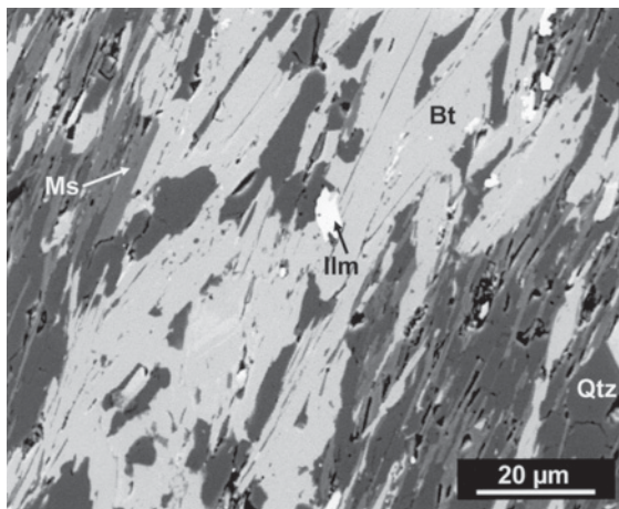
Figure 2. BSE image from an unshaped slate in the contact-metamorphism aureole. Bt: biotite; Ms: muscovite; Qtz: quartz; Ilm: ilmenite.
