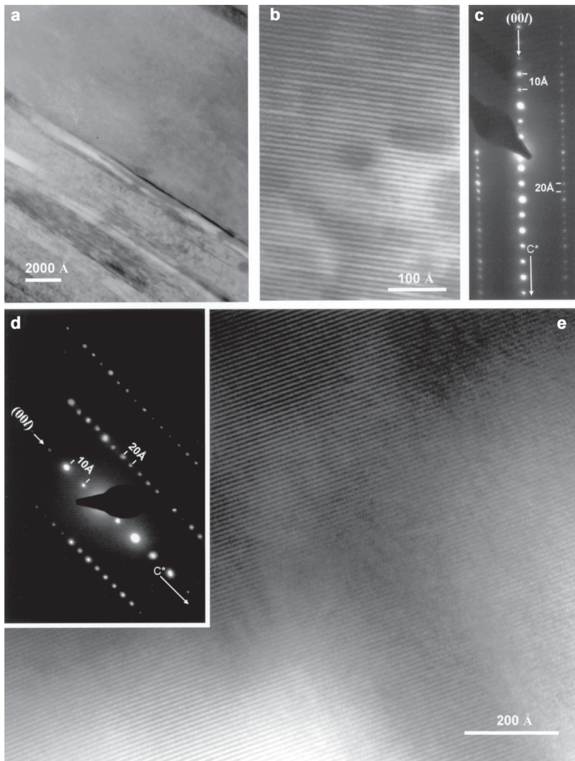
Figure 5. TEM images from contact-metamorphozed slates unaffected by the shear zone. (a) Low-magnification image showing biotite grains with sub-parallel packets. (b) Lattice-fringe image of a part of this biotite crystal. (c,d) SAED images recorded along \langle 100 \rangle / \langle 110 \rangle / \langle 1\bar{1}0 \rangle showing non-00l reflections with 20 Å periodicity. (e) Lattice-fringe image corresponding to SAED images shown in parts c and d.
