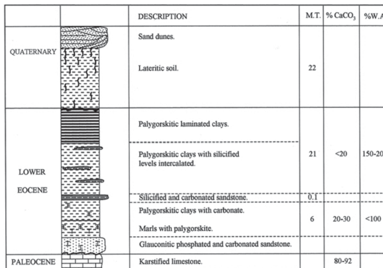
Figure 2. Schematic stratigraphic section of the Allou-Kagne deposit. M.T. = maximum thickness (m). W.A. = water absorption.
