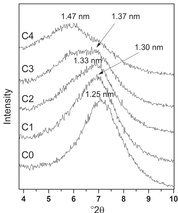
Figure 3. XRD patterns of oxidized or unaltered (oxidized) samples C0 to C4.
