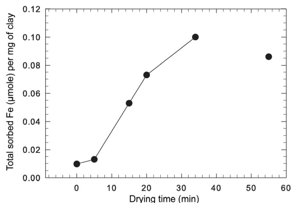
Figure 1. Amount of Fe sorbed on the SAZ-1 smectite film ( \mu\text{mole}/\text{mg} ) during preparation of the clay-modified Fe electrodes. Line added for clarity only. The point at 0 min drying time was achieved using the SAZ-1 suspension before it was applied to the Fe electrode. The point at 55 min of drying time was recorded after the electrode had been soaked in borate buffer for 5 min.
