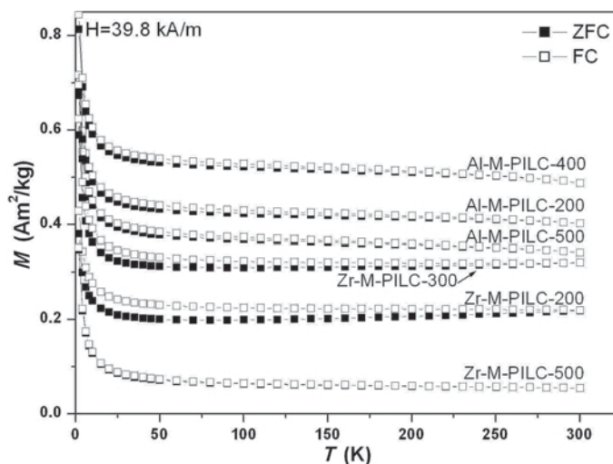
Figure 5. ZFC/FC curves of Al-M-PILC and Zr-M-PILCs. Filled symbols: ZFC; open symbols: FC curves.
