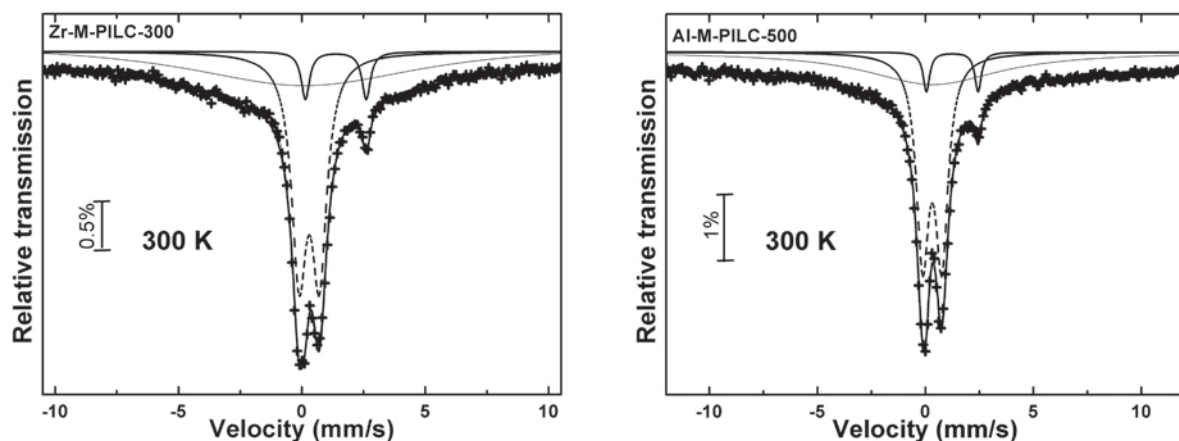
Figure 6. Room-temperature Mössbauer spectra of Al-M-PILC-500 and Zr-M-PILC-300.
