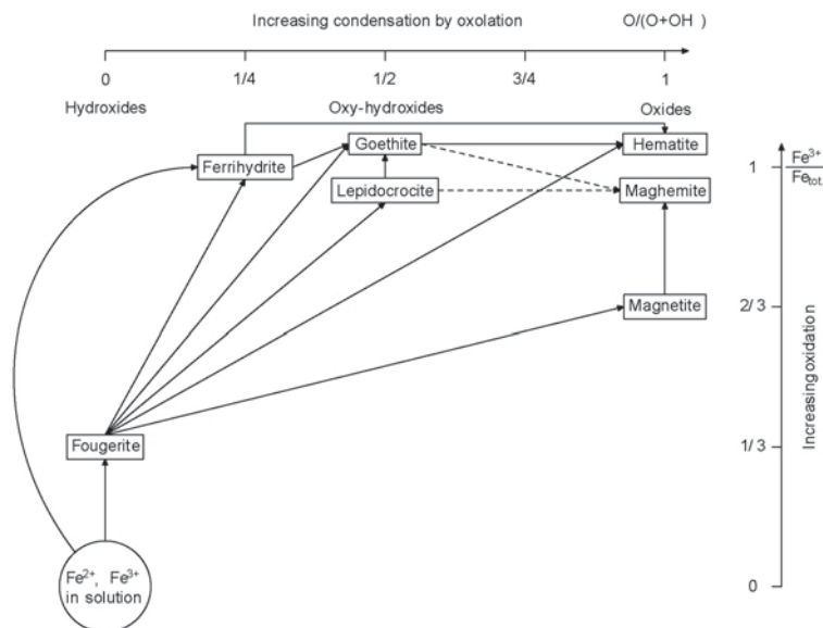
Figure 5. Location of fougerite in the pathways of formation of Fe oxides ( s.l. ). Abscissa: mole ratio O/(O+OH) , increasing condensation by oxylation from left to right. Ordinate: mole ratio of Fe^{3+}/Fe_{total} , increasing oxidation from the bottom to the top. Fougerite and ferrihydrite appear as key intermediate phases.
