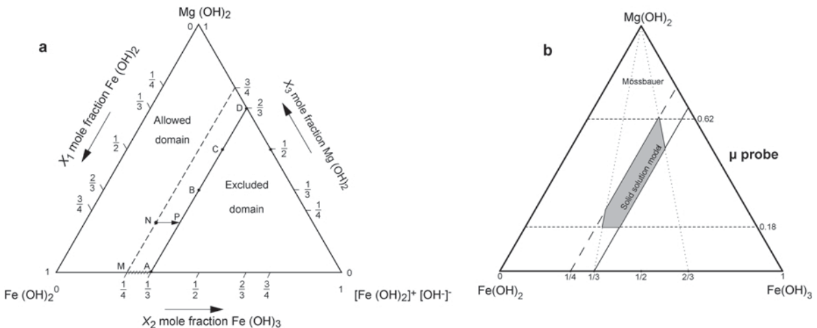
Figure 4. (a) Diagram for the ternary system \text{Mg}(\text{OH})_2 – \text{Fe}(\text{OH})_2 – \text{Fe}(\text{OH})_3 . Solid line: limit between the excluded domain and the domain allowed for stable ‘green rusts’ structure; dashed line: limit of the incipient precipitation of green rusts; from M to A on the horizontal axis: interval of the composition of synthetic green rusts; B, C and D: different compositions of green rusts; N \rightarrow P : oxidation path of fougerite. (b) Ternary diagram of the stability of fougerite derived from Mössbauer data (dotted lines), a solid-solution model (solid line and long dashed lines, see also Figure 4a), extraction by citrate-bicarbonate, and EMPA (horizontal short dashed lines). The limits of composition of fougerite from Fougères are given by the shaded area resulting from the intersections of those six straight lines.
