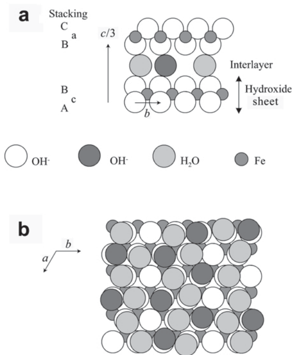
Figure 3. Proposed crystal structure of GR1(OH) for a chemical composition of [\text{Fe}_3^{\text{II}}\text{Fe}^{\text{III}}(\text{OH})_8]^+ [\text{OH}, 2\text{H}_2\text{O}]^- . (a) Stacking sequence; (b) positions of water molecules and OH − ions in an interlayer viewed along [001]. Relative sizes of ions are drawn to scale. One interlayer, one OH plane and one Fe plane are represented below.
