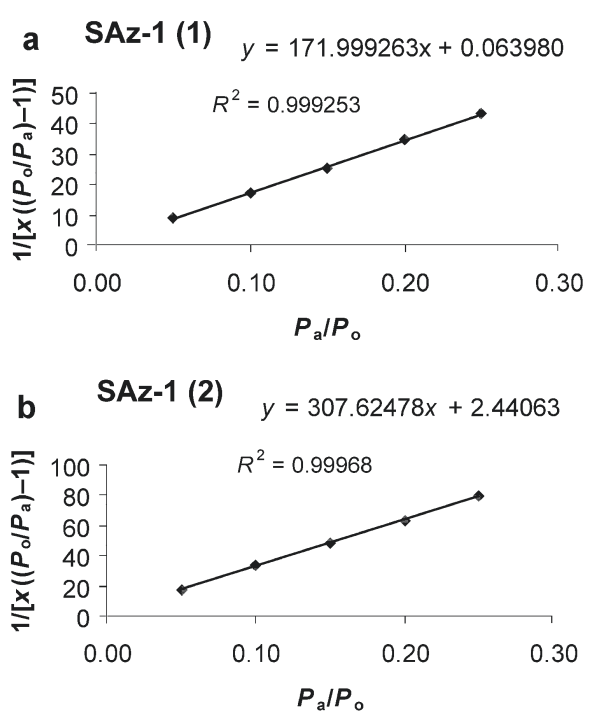
Figure 4. BET specific surface area measurement of the source clay SAz-1: (a) the first BET plot; and (b) the second BET plot.
