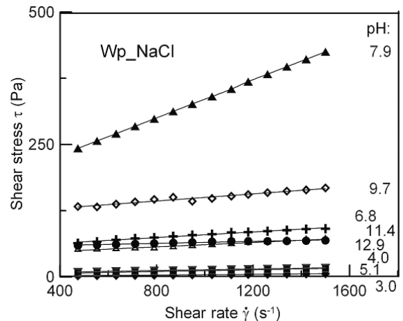
Figure 14. Flow curves of Wp clay suspensions in NaCl solutions at different pH values.
