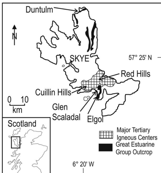
Figure 1. Map of the Isle of Skye showing the Tertiary igneous centers and the area where the Elgol marl samples were collected. The Great Estuarine Group rocks near Duntulm are dominated by smectite whereas illite is predominant in the rocks near Elgol (Andrews, 1987). Further information about the Elgol samples was provided by Woods et al. (2002). This figure is modified after Hudson and Andrews (1987).
