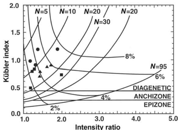
Figure 2. A plot of Kübler index vs. the Środoń intensity ratio for Elgol I-S. Isopleths (from Eberl and Velde, 1989) are of the XRD scattering domain size ( N ) of I-S crystallites and of the percentage of swelling (smectite) layers in I-S. Circles denote <0.25 μm fractions, triangles denote 0.25–1.0 μm fractions, and squares denote 1–2 μm fractions.
