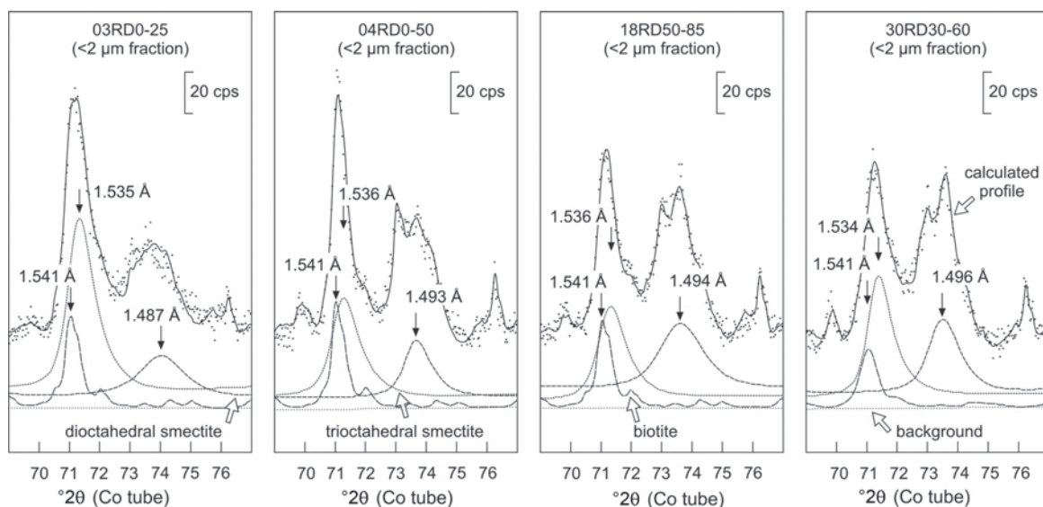
Figure 4. XRD patterns (random powder mounts, 69–77°2θ region) of the <2 μm fractions of the hydrothermally altered trachybasalt samples. Full-pattern fitting (points = measured data, solid line = fitted XRD profile) of the step-scan data was performed by the Rietveld method. The fitted profiles of dioctahedral and trioctahedral smectite as well as biotite are shown to illustrate the contributions of these phases to the overall diffraction profile, but all other phases were omitted for clarity. Note that the position and shape of the broad reflection centered at 1.54 Å cannot be described accurately without assuming the presence of trioctahedral smectite.
