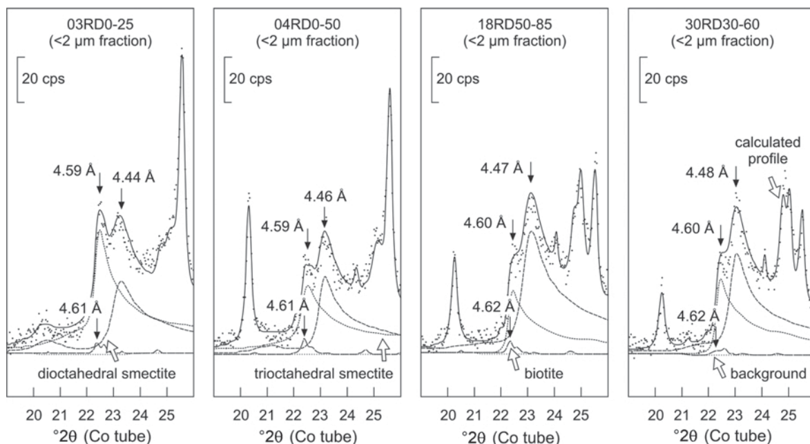
Figure 5. XRD patterns (random powder mounts, 19–26°2 \theta region) of the <2 \mu\text{m} fractions of the hydrothermally altered trachybasalt samples. Full-pattern fitting (points = measured data, solid line = fitted XRD profile) of the step-scan data has been performed by the Rietveld method. The fitted profiles of dioctahedral and trioctahedral smectite as well as biotite are shown to demonstrate the contributions of these phases to the overall diffraction profile. The fitted profiles of all other phases were omitted for clarity. Note that the broad 02,11 asymmetric band of the dioctahedral smectite at 4.45–4.46 Å has a shoulder at 4.59 Å that cannot be described accurately without assuming the presence of trioctahedral smectite.
