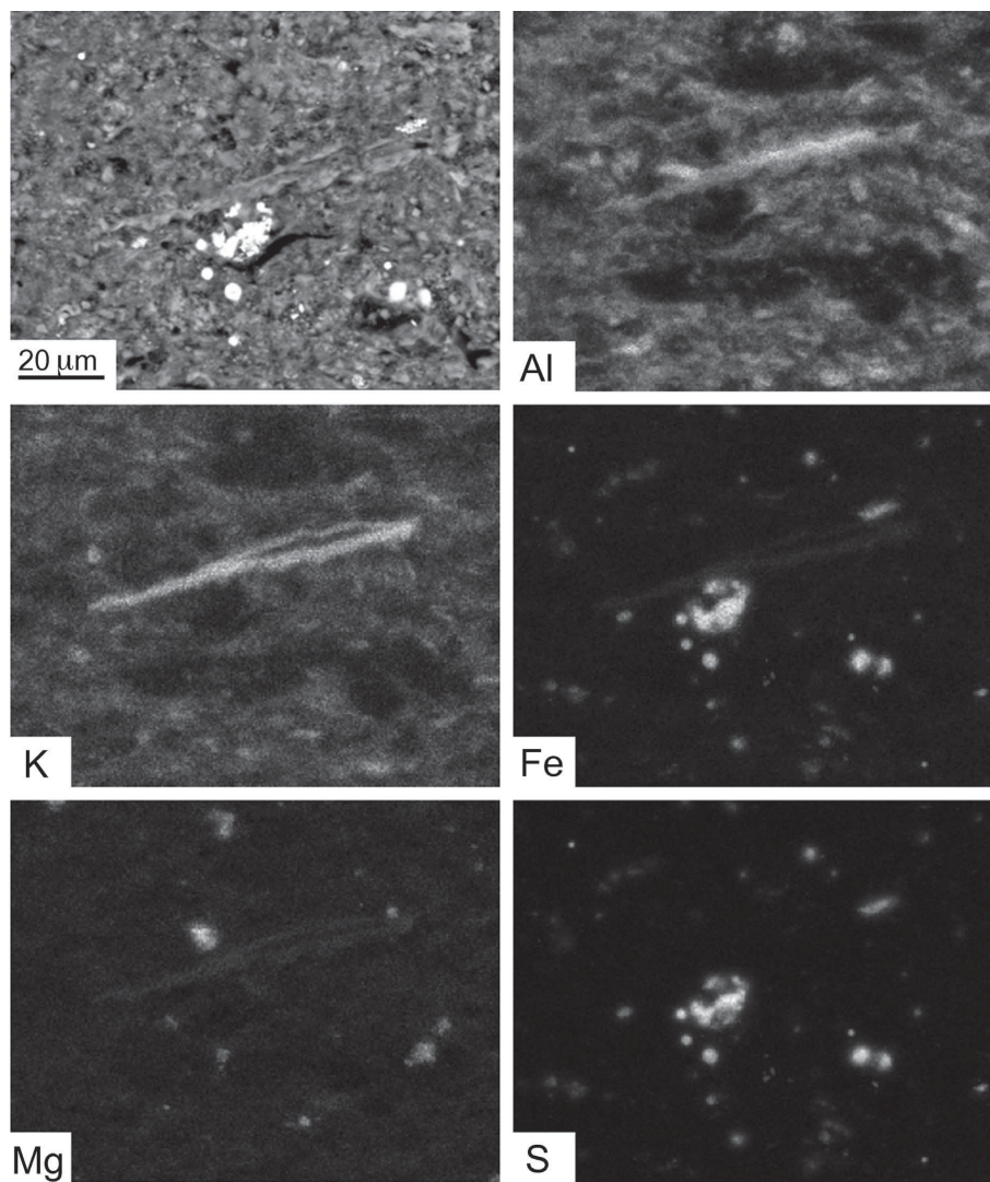
Figure 3. EDS analysis of sample S4 showing elemental maps of Al, K, Fe, Mg, and S, with an elongated illite-mica grain in the center.
