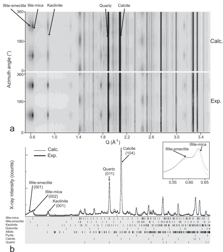
Figure 4. A comparison of (a) ‘unrolled’ diffraction spectra of sample S4 between the calculated model (upper) and the experimental data (lower) and (b) diffraction peaks in the spectrum which display eight constituent minerals. The variation in intensity along the azimuth are clearly displayed in (a) and are indicative of the preferred orientation for some minerals. The insert in (b) is an enlargement of the Q \sim 0.6 \text{ \AA}^{-1} peak showing the overlapping 002 peaks of illite-mica and illite-smectite. The dotted line represents experimental data and the solid line is the Rietveld fit extracted.
