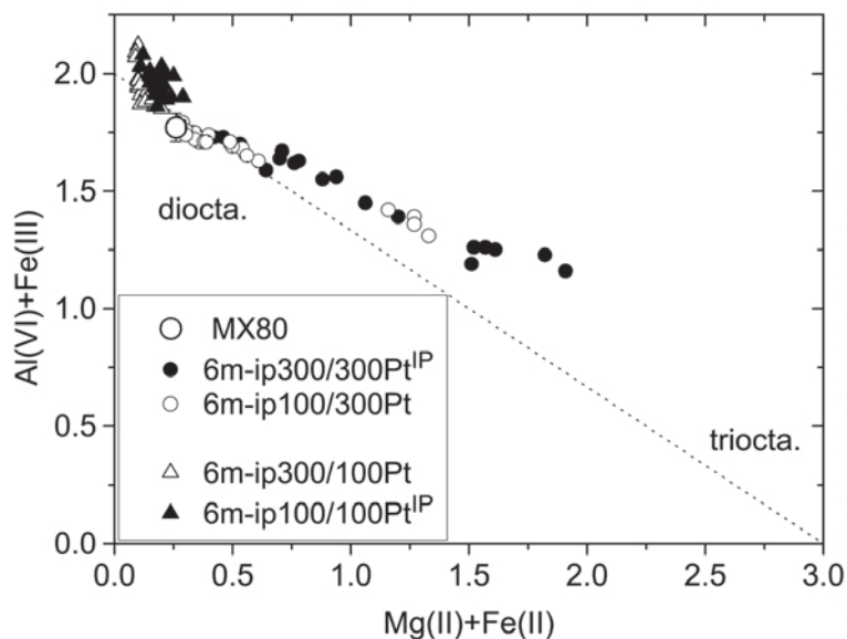
Figure 11. Evolution of the Fe oxidation state of the clay particles in samples 6m-ip300/300Pt, 6m-ip100/300Pt, 6mip300/100Pt, and 6m-ip100/100Pt. ^{VI}\text{Al} , Mg, and total Fe from TEM-EDS; Fe(III) to Fe(II) ratio from TMS. IP: position of the Fe plate; circles: hot parts; triangles: cold part; filled symbols: presence of an Fe plate; empty symbol: without Fe plate.
