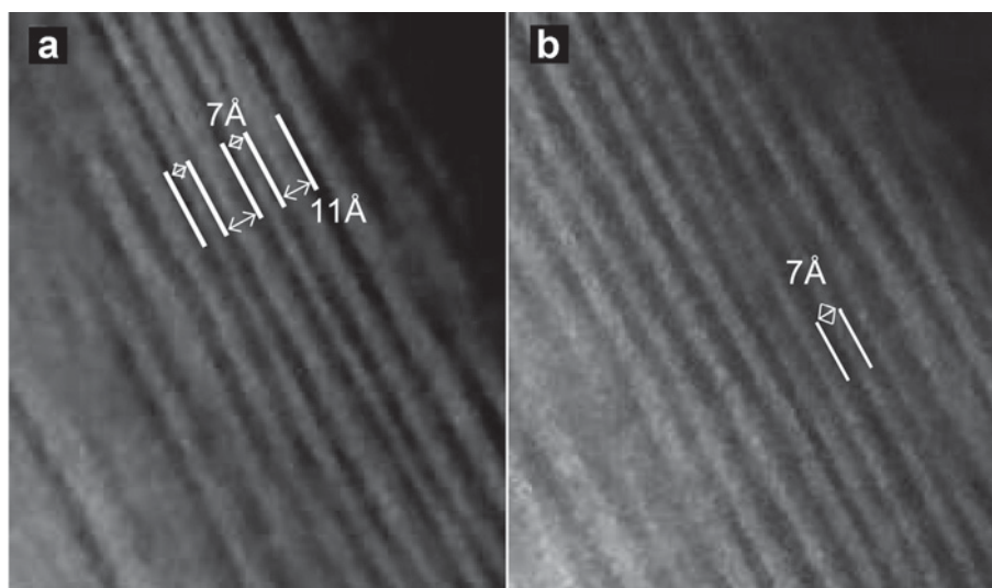
Figure 4. TEM images of the clay particles in sample 10m-ip300/300Pt. Small interlayer spacings (7 Å) alternate with 10–13 Å spacings (a) or form small groups (b).
