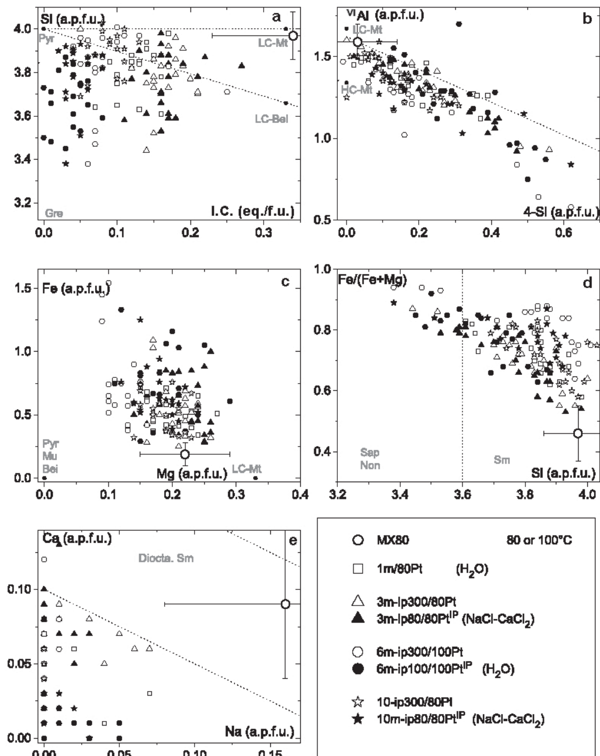
Figure 6. Crystal chemistry (from TEM-EDS) of the clay phase in the Pt capsules in the cold parts (100°C or 80°C) as a function of the position of the Fe plate and duration. Filled symbols indicate the presence of an Fe plate in the Pt capsule. IP: iron plate. (a) Si vs. I.C.; (b) ^{VI}Al vs. 4-Si; (c) Fe vs. Mg; (d) Fe/(Fe+Mg) vs. Si; (e) Ca vs. Na. See Figure 5 for symbol legend and axis units.
