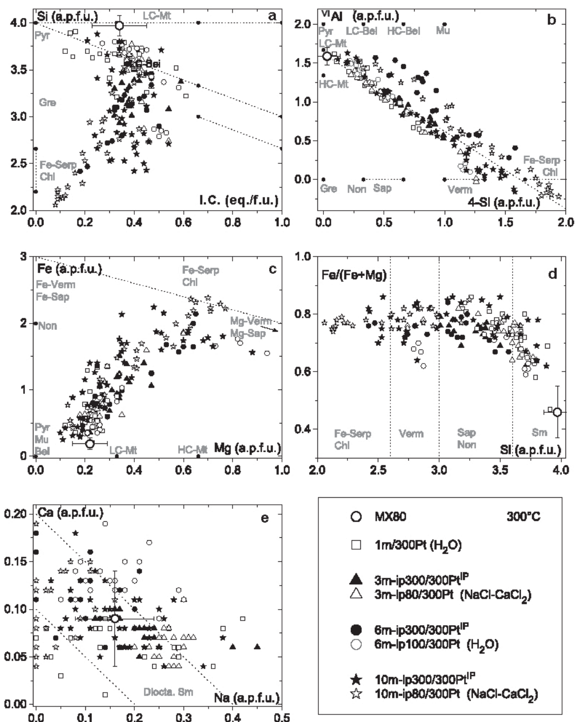
Figure 5. Crystal chemistry (from TEM-EDS) of the clay phase inside the Pt capsules in the hot parts (300°C) as a function of the position of the Fe plate and duration of the experiments. (a) Si vs I.C.; (b) VI Al vs. 4-Si; (c) Fe vs. Mg; (d) Fe/(Fe+Mg) vs. Si; (e) Ca vs. Na. Filled symbols: presence of an Fe plate in the Pt capsule. IP: Fe plate. Reference clays (Kostov, 1968; Caillère et al. , 1982): Bei: beidellite; Chl: chlorite; Fe-Serp: Fe-rich 7 Å phases; Gre: greenalite; Mt: montmorillonite; Mu: muscovite; Non: nontronite; Pyr: pyrophyllite; Sap: saponite; Sm: smectite; Verm: vermiculite; LC: low charge; HC: high charge; Al in octahedral sites VI Al = Al Tot - IV Al with IV Al = 4 - Si; interlayer charge I.C. = Na+K+2Ca. The dotted line in the diagonal of the 4-Si/ VI Al diagram indicates a constant total Al content. All structural formulae are calculated on the basis of the half unit cell, i.e. O 10 (OH) 2 . Other than for Fe/(Fe+Mg), the axis units are atoms per formula unit (a.p.f.u.) or atoms per half unit cell.
