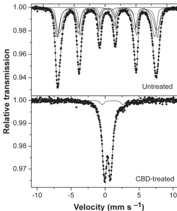
Figure 6. Effect of CBD treatment on Mössbauer spectra of 100% Fe-pillared Laponite at 4 K.
