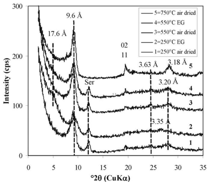
Figure 8. XRD traces of the smectitic clays heated at 250 and 550°C (oriented samples) and 750°C (random powders) for 90 min. EG = ethylene glycol solvation. Ser: serpentinite.
