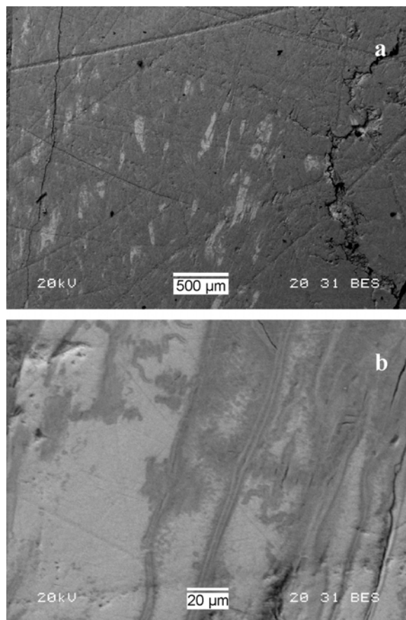
Figure 6. BSE images of the original smectitic clays.
