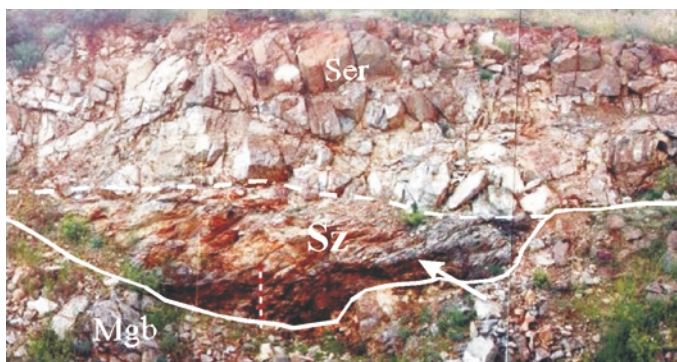
Figure 2. Development of the shear zone (Sz) at the contact between the serpentized plagioclase lherzolite (Ser) and microgabbro (Mgb). The exact location of the veinlets with smectite is indicated by the arrow. The vertical scale bar in the central bottom part is 1 m long.
