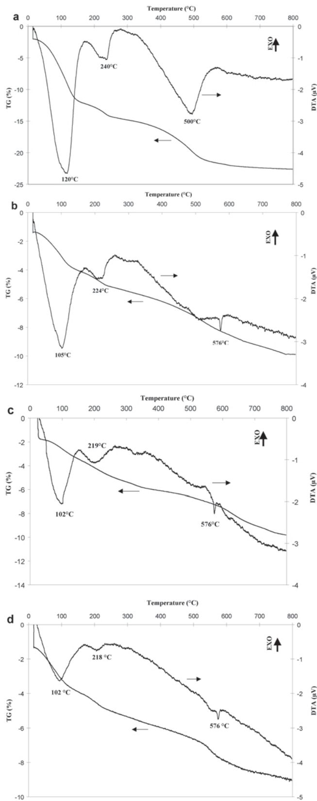
Figure 7. DTA-TG curves of: (a) starting soil; (b) sample from Z1; (c) sample from Z2; and (d) sample from Z3.
