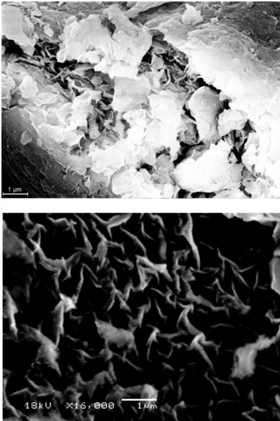
Figure 3. SEM images of smectite synthesized at 290°C.
