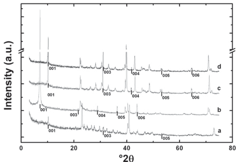
Figure 2. XRD patterns of the samples: a – muscovite, b – vermiculite, c – phlogopite, d – biotite; the 00/ diffractions are indicated directly under corresponding peaks.
