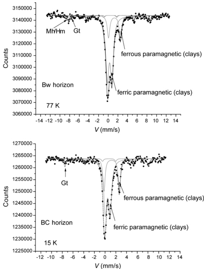
Figure 6. Mössbauer spectra of samples from Ascona I. Solid lines show individual fitting of components and their sum. Gt is assigned to goethite, Mh/Hm to hematite/maghemite mixtures.
