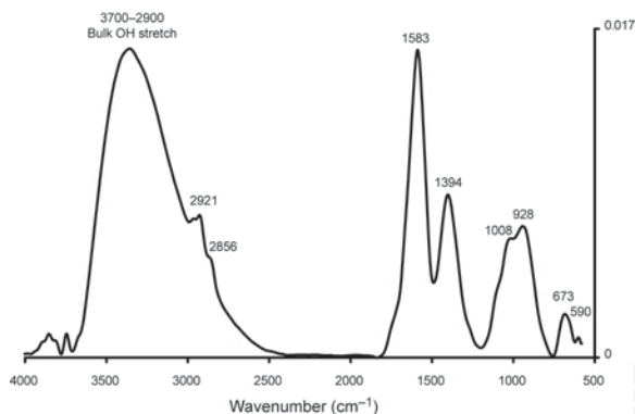
Figure 7. Conventional FTIR absorbance spectra of Fe film on a ZnSe window.
