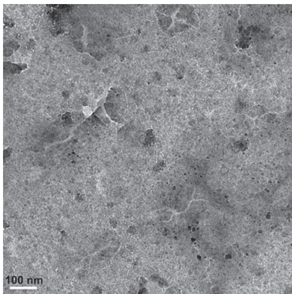
Figure 9. Bright-field TEM image of the Fe film.
