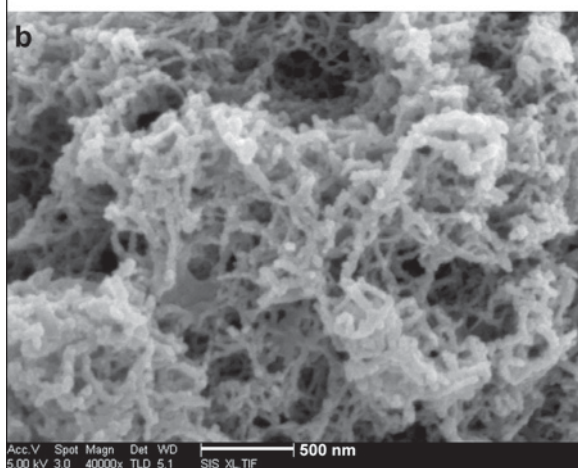
Figure 6. A HR-SEM image of the floccules. Sheath-like features (L?) may be Leptothrix sp. , based on \sim 2 \mu\text{m} diameter. (b) Increased magnification of (1) showing that floccules are made up of many small filaments which are much finer than bacteria cells. These may be dehydrated exopolysaccharides (e.g. Erlandsen et al. , 2004) or something similar.
