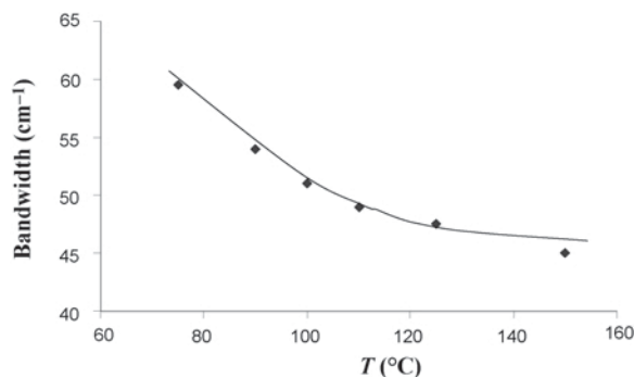
Figure 11. Width of the v\text{Fe}^{2+}\text{-OH} FTIR band of nontronite as a function of synthesis temperature. The band width is correlated to the crystallinity of nontronites.
