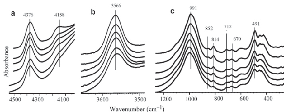
Figure 7. FTIR spectra of nontronites synthesized (from lowest to uppermost trace) at 75, 90, 100, 110, 125, and 150°C. (a) OH combination region; (b) OH-stretching region; (c) 1200–300 \text{cm}^{-1} region.
