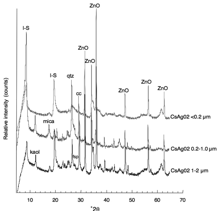
Figure 3. Random powder XRD patterns (CuK \alpha radiation) of different size fractions of the antibacterial CsAg02 clay, showing more detrital minerals in the coarser fractions, e.g. quartz (qtz), feldspar (fsp), calcite (cc), kaolinite (kaol).
