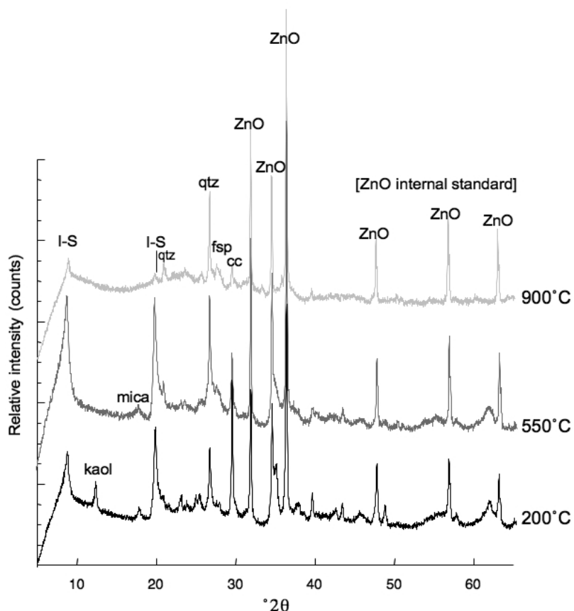
Figure 5. Random powder XRD patterns ( \text{CuK}\alpha radiation) of heated CsAg02 clay showing loss of smectite as the clay structure breaks down.
