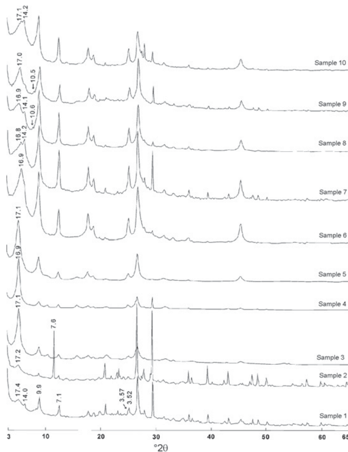
Figure 4. XRD patterns of the glycolated clays indicating that the clay comprises mixed-layer I-S, illite, chlorite, kaolinite and palygorskite in some of the samples. \text{CuK}\alpha radiation.
