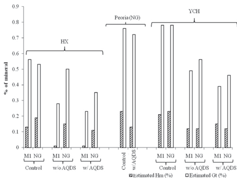
Figure 4. DRS estimate of goethite and hematite contents in un-reduced and bio-reduced loess samples. HX shows a decrease in hematite and goethite; Peoria shows a reduction in both hematite and goethite; and YCH shows a decrease in hematite and goethite after bio-reduction (w/o: without; w: with; HM; hematite; Gt: goethite).
