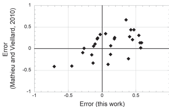
Figure 3. Comparison of errors (%) in \Delta H_f^\circ estimates (Table 6) using the polymer model (this study) and the electronegativity-based model of Mathieu and Vieillard (2010). Brewsterite data not shown (Table 6).
