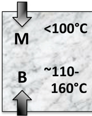
Figure 14. Diagram of possible beidellite formation: beidellite (B) generally precipitates from geothermal fluids entering a system from below, while montmorillonite (M) normally forms at lower temperatures, often where cool water enters the system from above.
