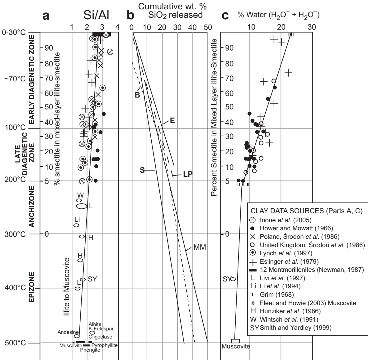
Figure 1. (a) Plot of Si/Al vs. temperature for the smectite-illite series, muscovite, and feldspars. Essentially, there is a regular decline of Si/Al from smectite to muscovite through the mixed-layer illite-smectite transition. For the smectite-illite series, scatter along the linear trend may be due to some clays being more aluminous than others of similar gross composition. Scatter may also be due to the presence of quartz impurity in the clay analyzed. The temperatures and diagenetic and metamorphic zones are from Merriman and Frey (1999). (b) The evolution of silica with increasing temperature, calculated in wt.% (see text), from the smectite-muscovite series. Published estimates plus those from this study are shown. Line B indicates the 20% illite/80% smectite of Boles and Franks (1979) altered to illite and muscovite; see text for calculated estimates. Line E is for smectite to illite from Eslinger et al. (1979). LP is the smectite to illite alteration as indicated by Leder and Park (1987). Line S indicates estimated silica released from montmorillonite altered to 94% illite from Środoń et al. (1986) and thence to muscovite. MM represents estimated silica evolved in the smectite to muscovite transformation. (c) Total water content ( H_2O^- plus H_2O^+ ) plotted for smectite-illite and muscovite illustrating the decrease in water over the range from smectite to illite and muscovite. Note that in the range of \sim 30^\circ\text{C} to 200^\circ\text{C} , \sim 70\% of the water originally contained in smectite is lost.
