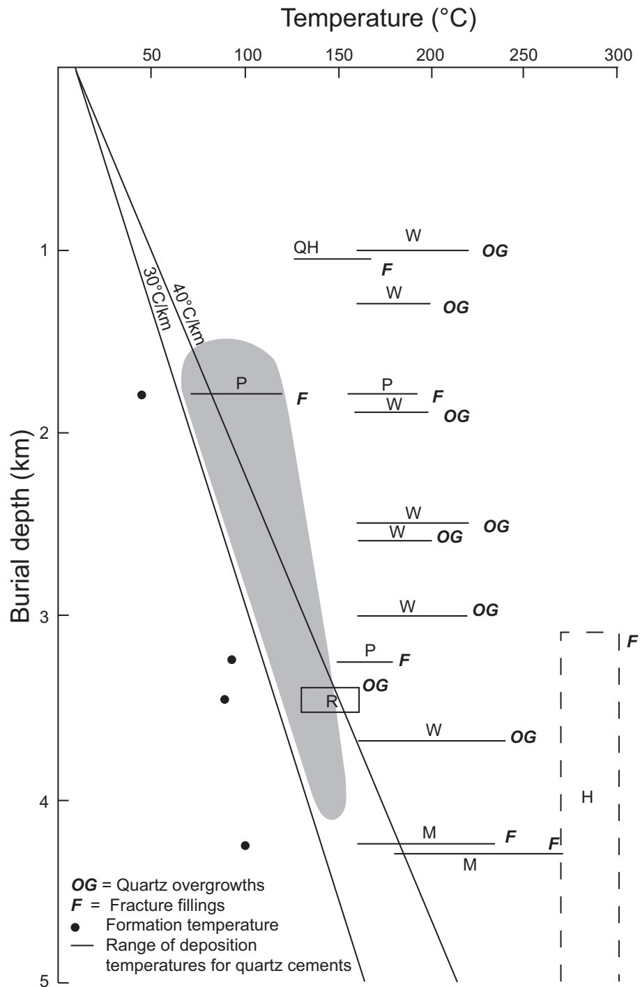
Figure 3. Fluid-inclusion homogenization temperatures for quartz overgrowths on detrital quartz grains and fracture fillings in sandstones plotted against maximum burial temperatures at their sites of deposition. The shaded area is the field of fluid-inclusion homogenization temperatures for quartz cements in many sandstones from Gluyas et al. (1993). Many inclusion temperatures are far greater than the ambient formation temperatures suggesting that the secondary quartz was transported in solution from a hotter source. For sedimentary basins, this source is inferred to be basinal shales buried deeper and hotter downdip from the sandstones in which the high-temperature cements were deposited. The apparent movement of silica in solution over vertical distances of 1 km or more implies major mass transfer. Letters above lines representing temperature ranges are for data sources as follows: H = Harrison et al. (2004), M = Mitcheltree (1997), P = Parnell et al. (2001), QH = Quinn and Haszeldine (2004), R = Rossi et al. (2002), W = Wycherly et al. (2003).
