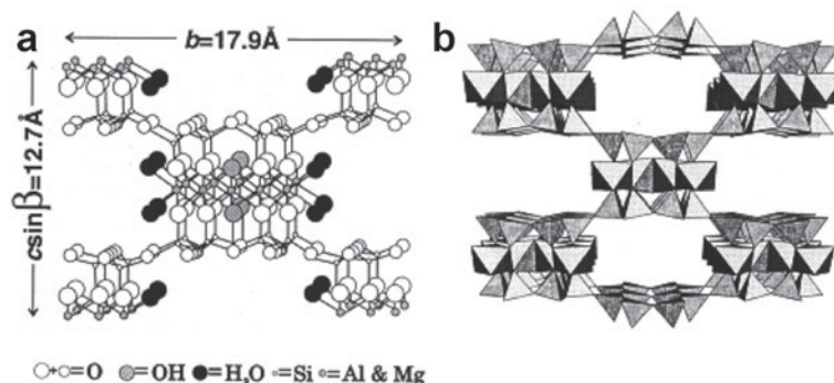
Figure 1. (a) Crystal structure of attapulgite (Bradley, 1940) and (b) its polyhedral representation (Mckeown et al. , 2002).
