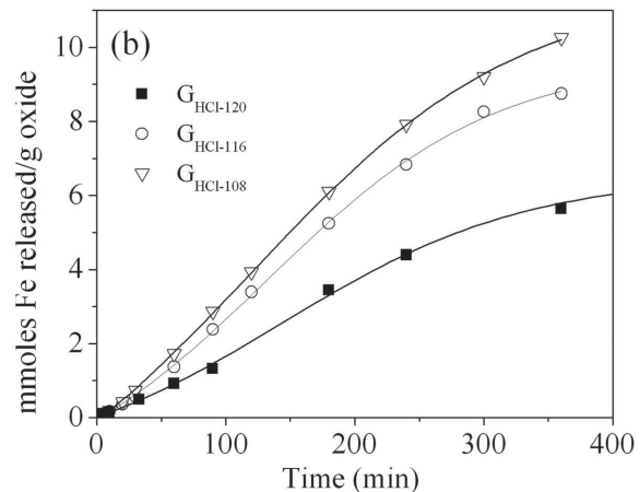
Figure 5. Representative dissolution curves for series (a) G_{ox-i} and (b) G_{HCl-i} , expressed as mmoles of Fe dissolved g^{-1} of oxide in 4 M HCl at 40°C vs. time.
