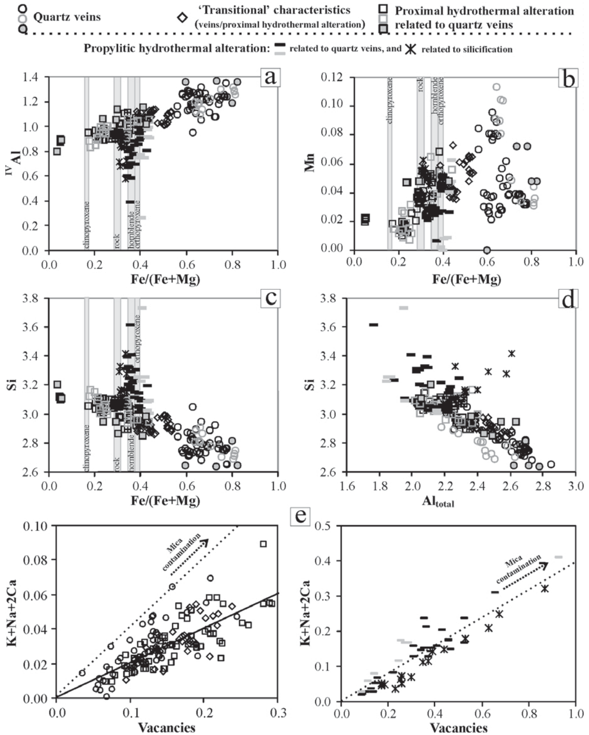
Figure 4. Binary diagrams showing compositional variations, expressed as atoms per formula unit (a.p.f.u.), between tetrahedral and octahedral cations and interlayer cations and vacancies in the different types of chlorites. Fe/(Fe+Mg) ratio data of the unaltered volcanic rock and phenocrysts (from Fernández Soler, 1996), which host the Palai-Islica deposit, are shown. EMPA analyses are plotted as open symbols, TEM-AEM analyses in gray-filled symbols, and SEM analyses as gray, open symbols. The influence of mica contamination and the correlation line in chlorite analyses are shown by dotted and solid lines, respectively (e).
