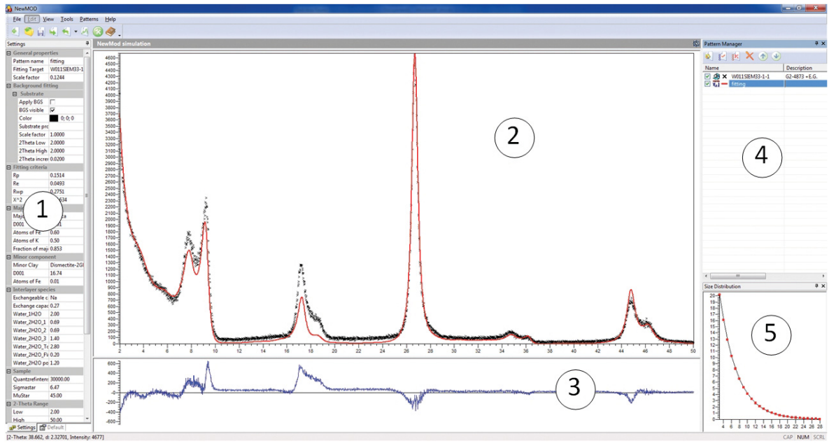
Figure 2. Layout of the Integrated Simulation Environment (ISE) of NEWMOD+. ①. Parameter panel contains all input parameters for NEWMOD+ as well as the graphical evaluation parameters R_p , R_{wp} , R_{exp} , and \chi^2 . ②. The working window plots both experimental and simulated profiles (the simulated pattern with solid curve is superimposed on the experimental pattern with cross symbol), the solid line at the bottom is the background profile. ③. The difference plot shows the difference between experimental and simulated profiles, thereby providing a graphical representation of the goodness-of-fit. ④. Pattern manager in which the investigator can manipulate the pattern with operations such as delete and change the visualization styles for the pattern, including colors and continuous line or dot. ⑤. Size distribution plot shows the crystal-size distribution characteristics for the current simulated pattern.
