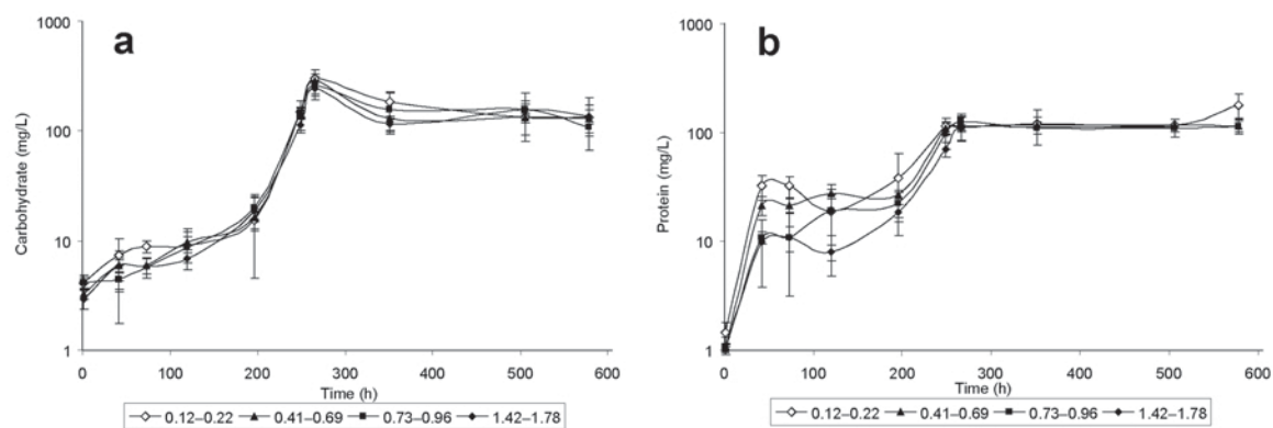
Figure 3. Time-course production of the carbohydrate (a) and protein (b) fraction of exopolysaccharide produced by CN32 cells during Fe(III) bioreduction.
