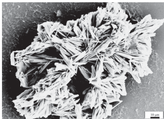
Figure 10. SEM image showing aggregated particles of chemically reduced nontronite. Most clay plates are aggregated in face-to-face and face-to-edge orientations.
