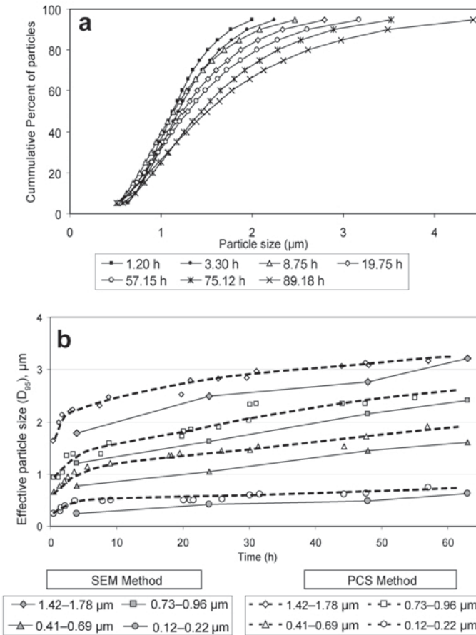
Figure 1. (a) Change in the distribution of particle size of the 1.42–1.78 μm fraction over the course of bioreduction (90 h). The size distribution was measured by the PCS method. (b) Change in particle size at 95% percentile ( D_{95} ) with time for four size fractions used in this study. The dotted lines represent the data obtained by the PCS method and the solid lines are those by the SEM method. The experiments were performed with 25 mM of Na pyrophosphate without shaking. The dotted lines are shown to elucidate the data trend, and are not model fits.
