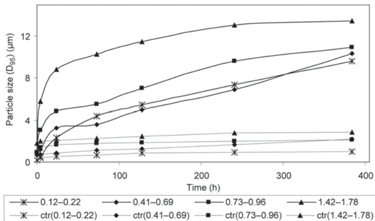
Figure 6. Time-course change in nontronite particle size at 95% percentile ( D_{95} ) (as measured by SEM) to illustrate more clearly the rate of nontronite particle aggregation during Fe(III) bioreduction. The data were taken from Fig. 5. The ctr symbols denote abiotic control.
