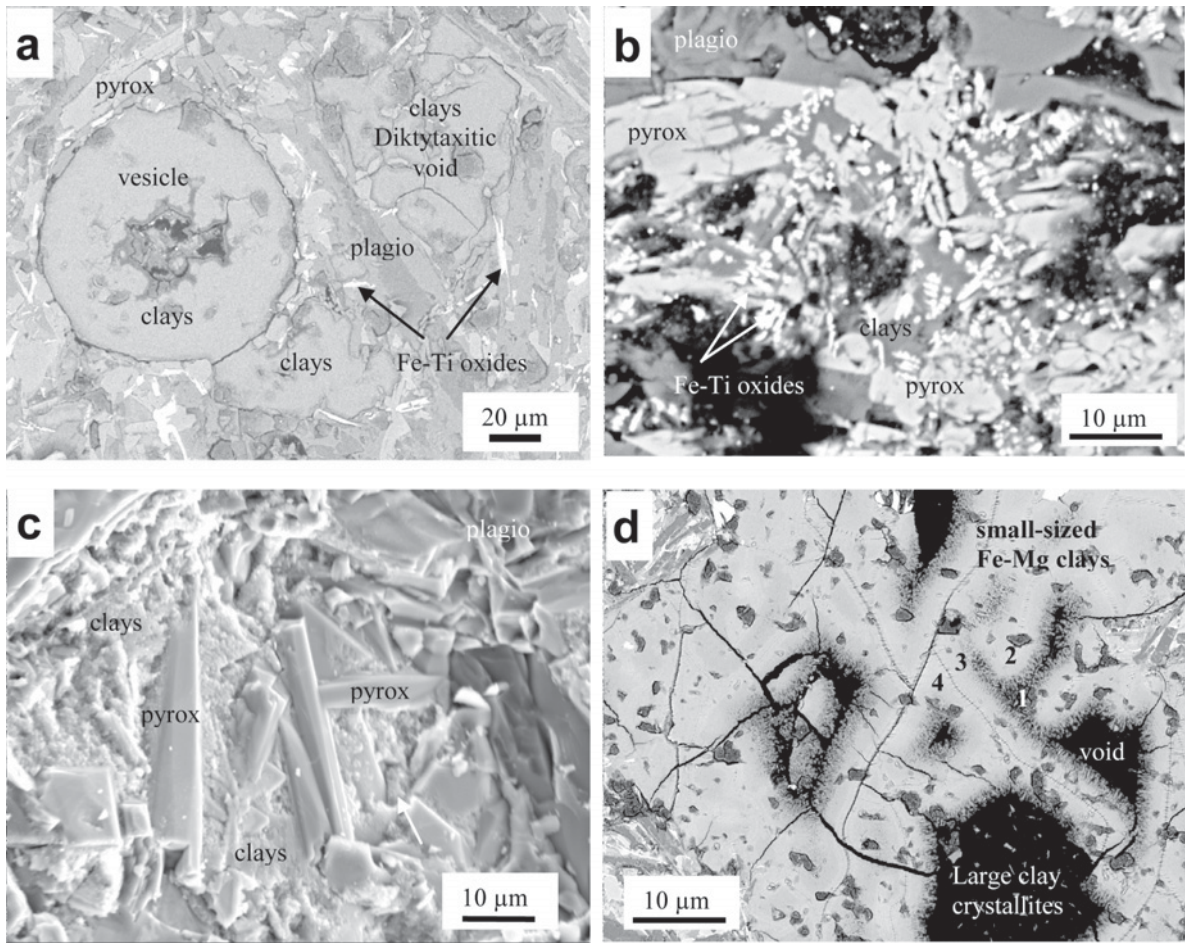
Figure 4. Submarine flow. SEM images of diktytaxitic voids and an olivine phenocryst. (a) BSE image showing the connection between a vesicle and the diktytaxitic voids. (b) BSE image of a black mesostasis formed of numerous Fe-Ti oxides scattered in a clay matrix. (c) SEM image of a diktytaxitic void showing the presence of euhedral pyroxene microcrysts embedded in a randomly oriented clay matrix. (d) BSE image of an olivine phenocryst pseudomorphosed by clay minerals. Numbers indicate the zones analyzed (Table 4).
