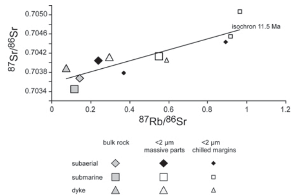
Figure 9. Relationship between the ^{87}Sr/^{86}Sr and ^{87}Rb/^{86}Sr ratios for the bulk rocks and the <2 μm fraction extracted from the massive parts and the chilled margins of the three volcanic bodies. The line represents the 11.5 Ma isochron.
