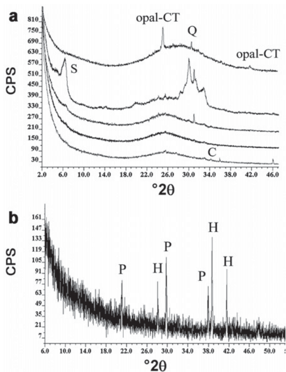
Figure 4. XRD patterns of sinter from each zone: (a) opal-A is represented by the broad central peak around 25^\circ 2\theta or 4.03 \text{ \AA} . The upper pattern is of the spicular zone, then altered, crustal, dark/light laminated, and dark laminated at the bottom. Opal-CT, smectite (S), quartz (Q), and calcite (C) were also identified. (b) Dark mm-sized grains of pyrite (P) and hematite (H) found within the altered zone. CoK\alpha radiation.
