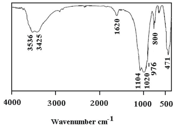
Figure 4. IR spectrum of glauconitic material.
