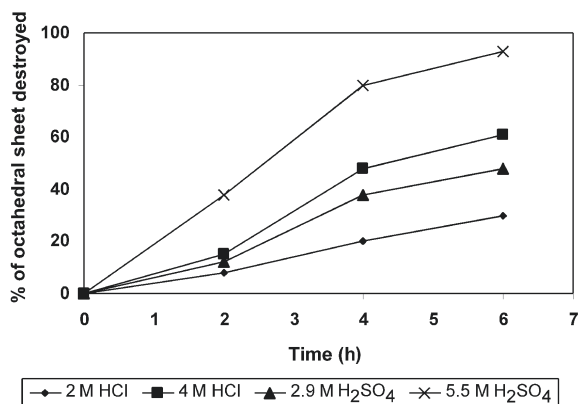
Figure 8. Ratio of decomposed octahedral sheets (%) as a function of acid concentration and leaching times.
