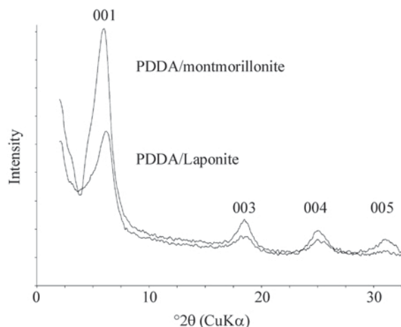
Figure 4. XRD patterns comparing the intensities of reflections in ~100 nm thick films of PDDA/montmorillonite (upper) and PDDA/Laponite RD (lower) at low RH (25% for PDDA/montmorillonite and 23% for PDDA/Laponite RD). The vertical axis shows the square root of intensity.
