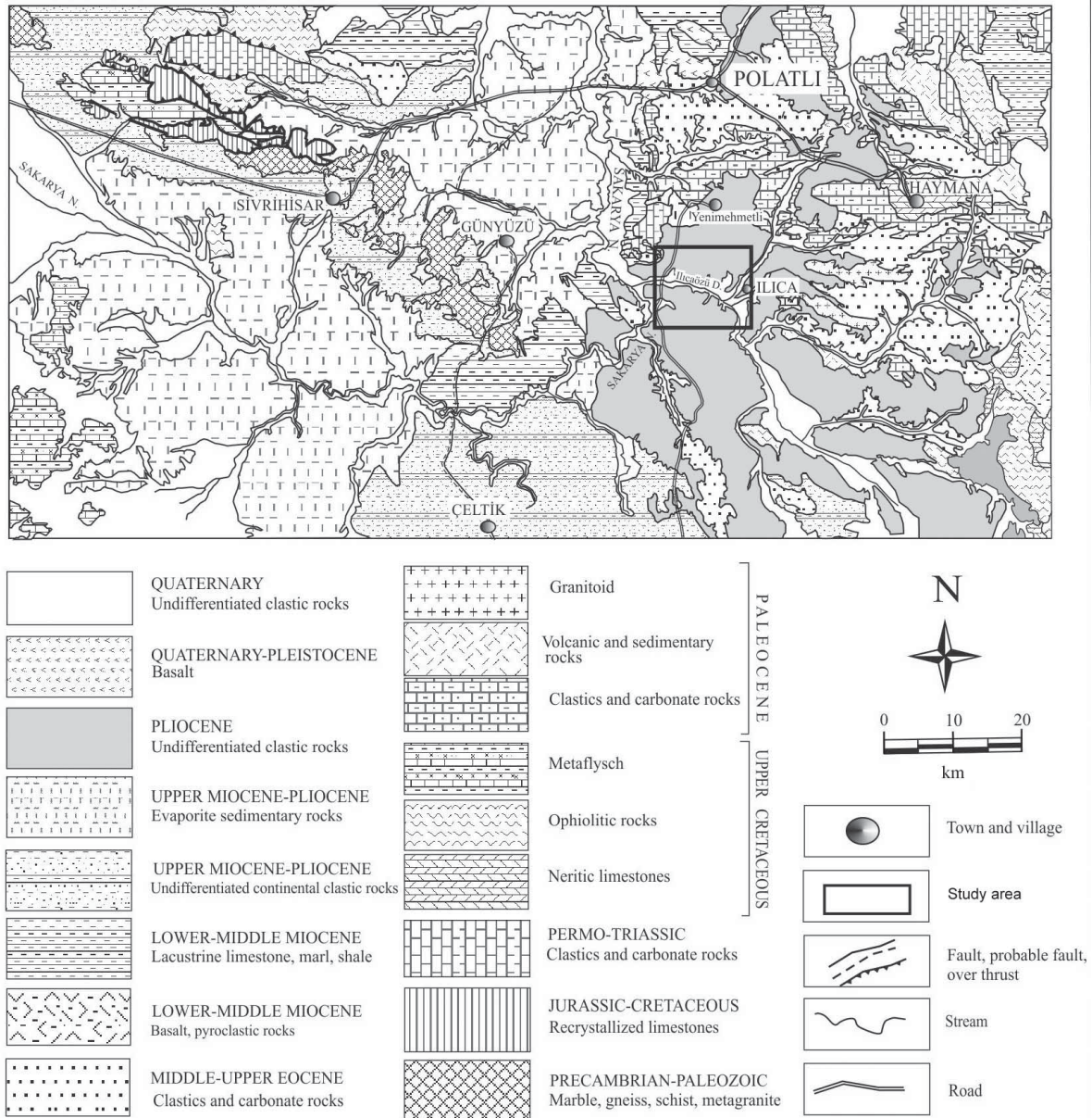
Figure 1. Detailed geologic map of the Sakarya basin, central Anatolia, Turkey (simplified from a 1:500,000 scale map – MTA, 2001).
