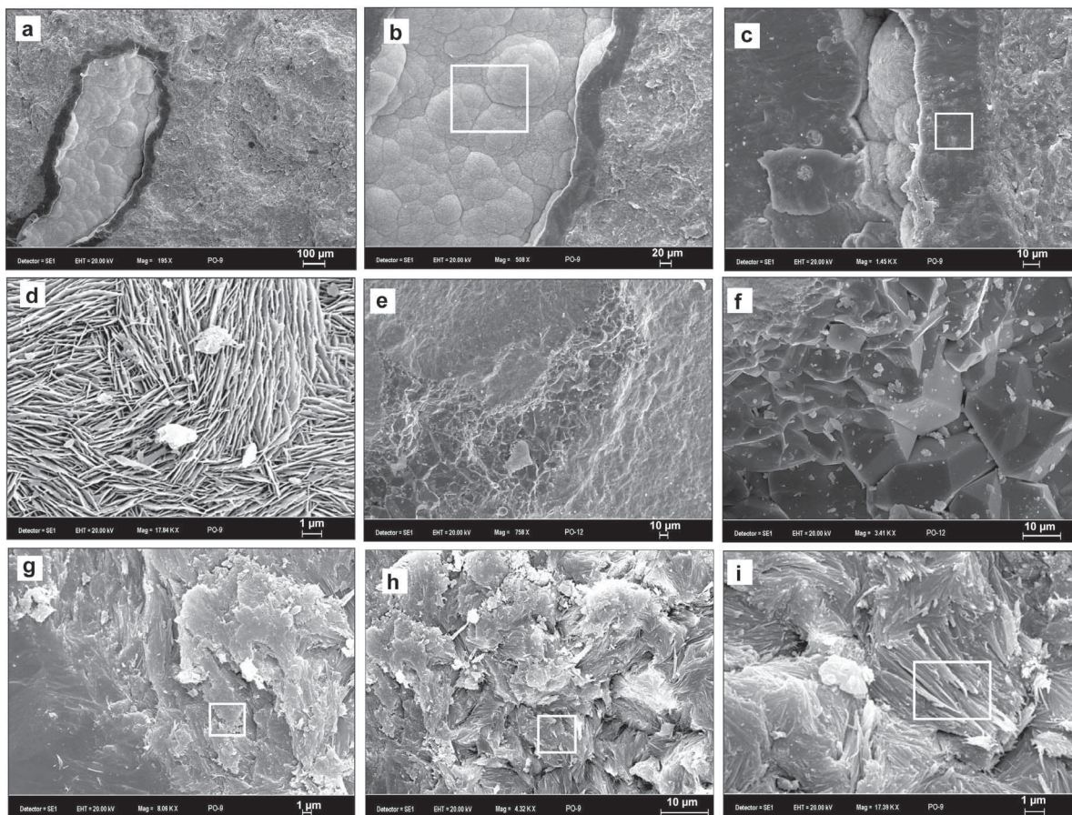
Figure 7. (a–c) Opal and quartz (chalcedony) were found in cavities of the sepiolitic claystone. The spherical particles of amorphous silica with a diameter of \sim 0.5 – 100 \mu\text{m} are tightly packed with botryoidal opal-A and opal-CT lepispheres. The lamellae containing crystalline silica generally display an amorphous rim with a diameter of 5 – 30 \mu\text{m} , and the crystalline area has a characteristically uniform contrast. (d) Aggregated small, hexagonal, blade-shaped quartz crystals are also seen. (e, f) Several platy silica particles show a continuous transition between amorphous silica (opal-A) and crystallized silica (opal-CT-quartz). The particles are composed of several closely stacked, thin lamellae, with pseudo-hexagonal shapes and diameters of 200 – 300 nm across. The opal-CT is converted to quartz. (g–i) In the globular grains, long, thin fibers of sepiolite show progressive transformation to short and thick (Mg-poor) sepiolite fibers to opal-CT to euhedral quartz.
