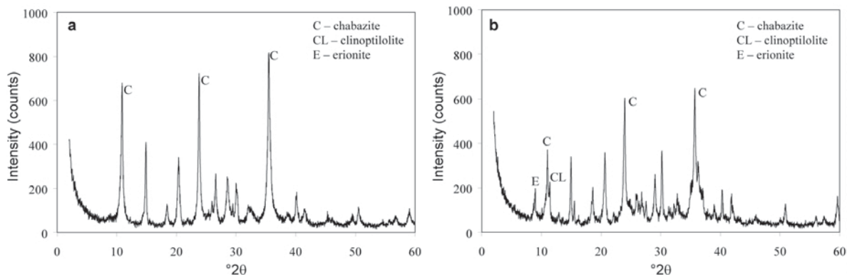
Figure 2. Powder XRD patterns of the: (a) synthetic chabazite analog; and (b) mineral chabazite.
