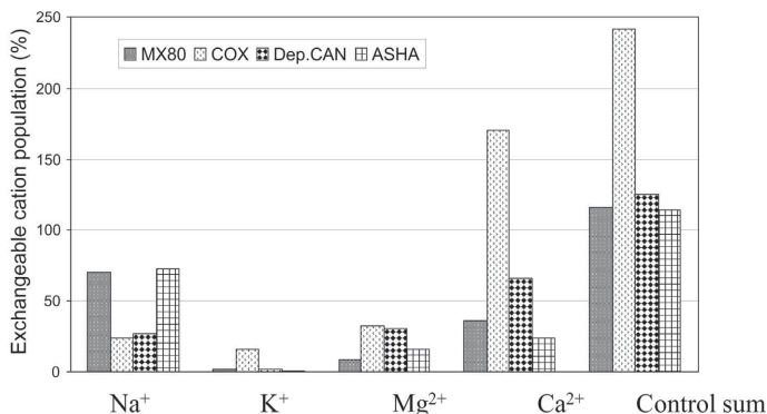
Figure 4. Calculated exchangeable cation population (%) with respect to CEC (VIS).
