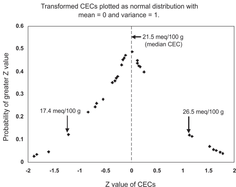
Figure 1. CEC values reported by iSE (2006) were standardized to normal distribution using the instructions and the Z value vs. probability table of Steel and Torrie (1980). (Z value = standard score which indicates by how many standard deviations the value is above or below the mean.) The CEC values with Z > 1 or Z < -1 can be deemed questionable.
