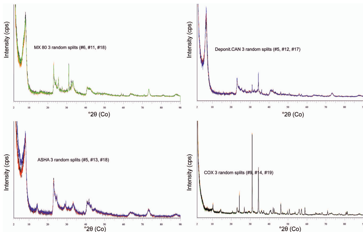
Figure 2. XRD patterns of three random splits of MX 80 (upper left), Deponit.CAN (upper right), ASHA (lower left), and COX (lower right). The patterns were superimposed to identify intensity differences.
