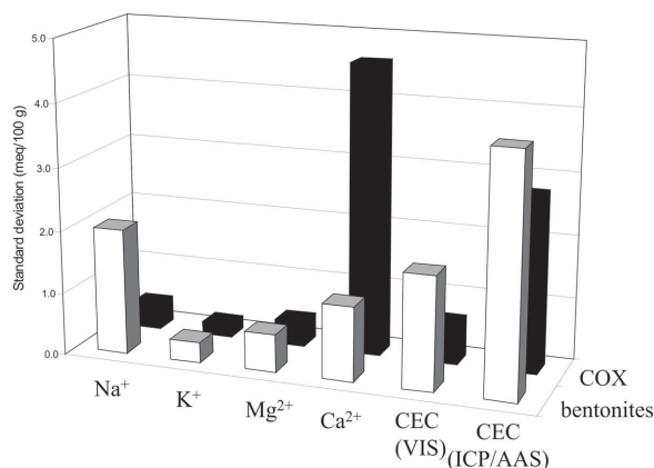
Figure 3. Precision (standard deviation) of exchangeable cations and CEC values.
