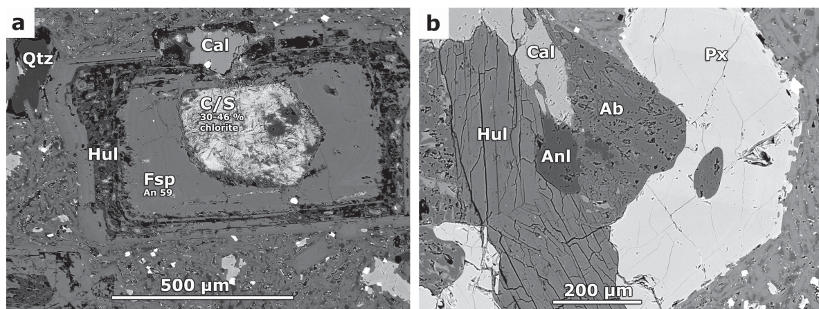
Figure 2. Backscattered electron (BSE) images from outcrop Z57: (a) plagioclase feldspar (Fsp) being replaced by heulandite (Hul) with C/S part of a previously mafic magmatic mineral. (b) Sample with analcime (Anl) together with heulandite (Hul), calcite (Cal), albite (Ab), and clinopyroxene (Px).
