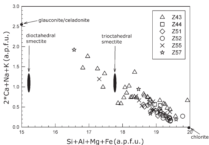
Figure 4. Composition of mafic phyllosilicates in basalts from the Balșa-Techereu-Poienița area, normalized to 28 oxide charge equivalents. The total moles of charge of exchangeable cations ( 2 \times \text{Ca} + \text{Na} + \text{K} ) are plotted as a function of the total molar ( \text{Si} + \text{Al} + \text{Mg} + \text{Fe} ) content. Ideal end-member compositions of chlorite, celadonite (filled circles), trioctahedral smectite, and dioctahedral smectite (filled ovals) are also depicted.
