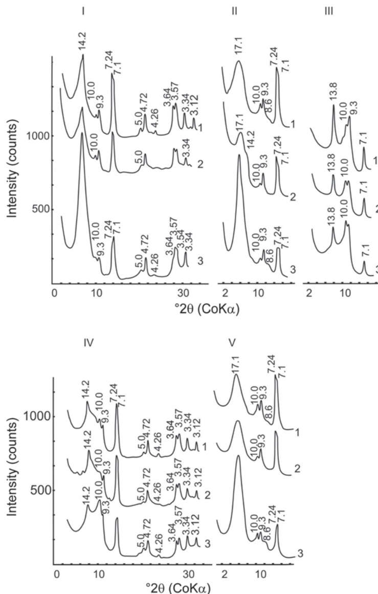
Figure 3. XRD patterns of the <1 \mu\text{m} fraction of Pit Y-02-07: (I) Mg-saturated; (II) ethylene glycol-solvated; (III) 350^\circ\text{C} ; (IV) 350^\circ\text{C} + ethylene glycol; (V) 550^\circ\text{C} . Horizons: (1) Ah (0–4 cm); (2) Bg (4–15 cm); (3) Bgf (15–30 cm).
