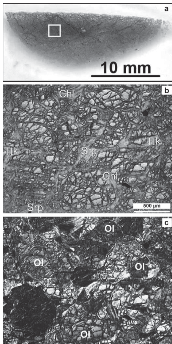
Figure 2. (a) Thin, polished section of serpentinite. The white box indicates the area of study. (b,c) Reticulate structure of olivine grains (Ol), substitution by aggregate veins of serpentine (Srp) by talc (Tlk) and chlorite (Chl). Veins make up a net with relict fragments of olivine grains in loops (b: plain polars; c: crossed nicols).
