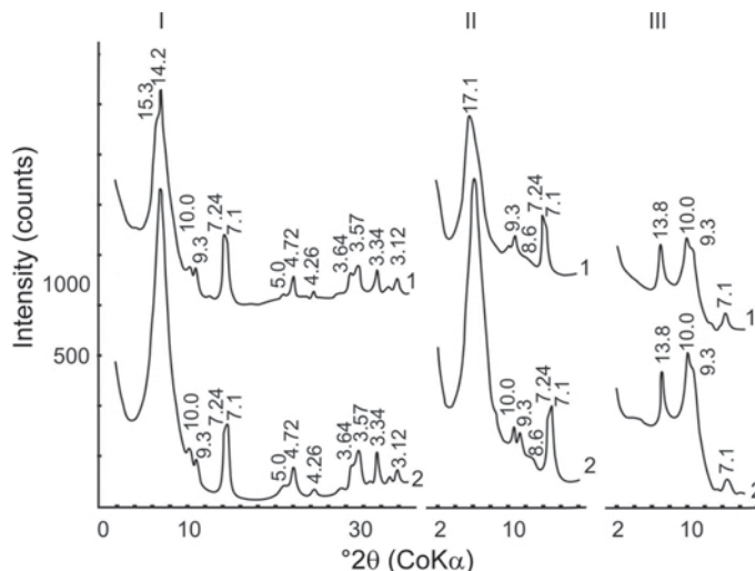
Figure 5. XRD patterns of the <1 \mu\text{m} fraction of Pit Y-03-07. (1) Mg-saturated; (II) ethylene glycol-solvated; (III) 550°C. Horizons: (1) Bg (0–10 cm); (2) Bgf (10–20 cm).
