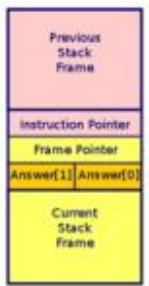
Figure 1 An example Call Stack with gsubmit local variables (Answer) explicitly displayed. Note that this stack grows down.
